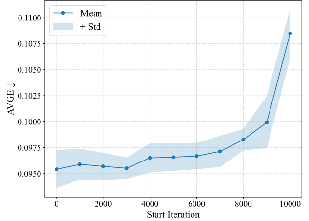
Figure 9. Ablation study on the application phase. We show the improvement of applying our method during the final N\% of total training iterations.
